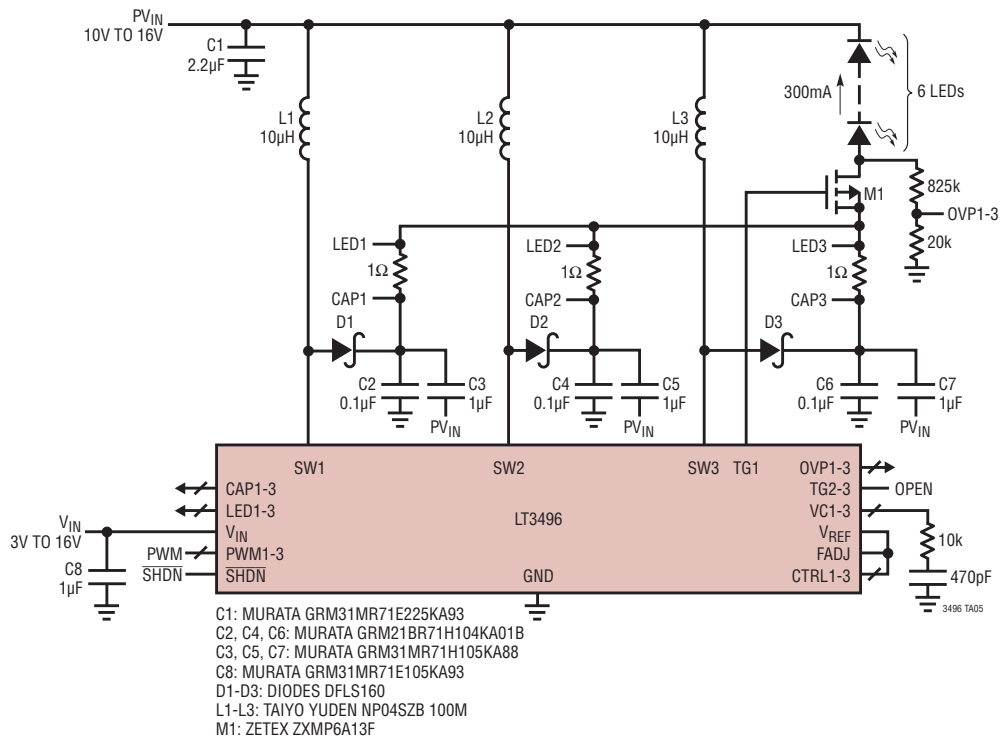
Buck-Boost Mode 300mA × 6 LED Driver
